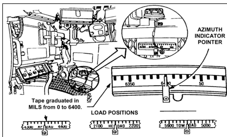
Figure 7-10. Azimuth indicator.
